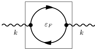
Fig. 1. Lowest order vacuum polarization diagram.
