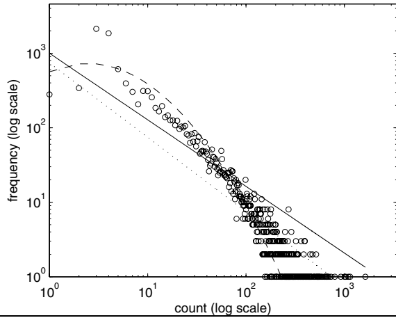
Figure 16. MS distribution and fitted curves for Tomcat.
