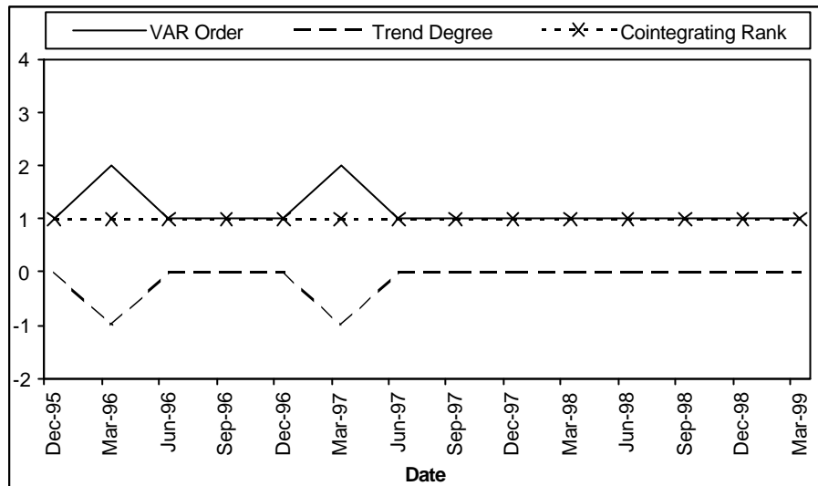
Figure 3: Multivariate evolving model selected by PIC-RRR.
