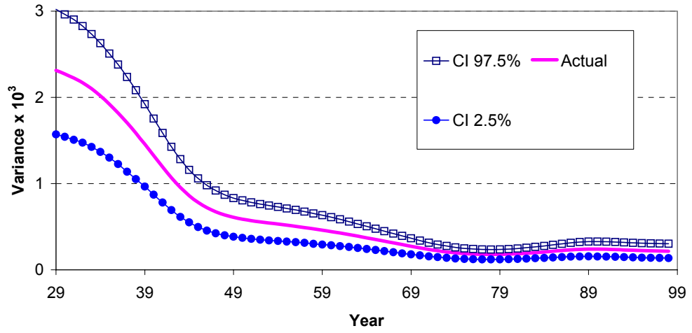
Figure 7: Time Path of \hat{\sigma}_t^2 with Bootstrap Confidence Interval for the 48 US States Panel.
