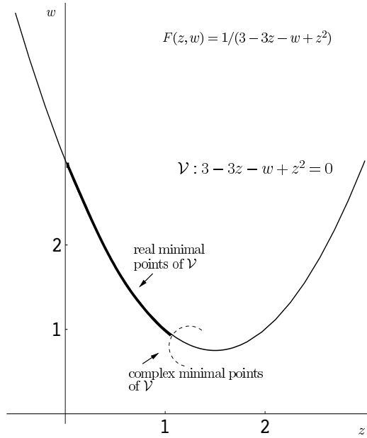
FIGURE 2. \mathcal{V} for Example 3.4
