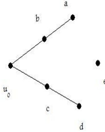
Figure 7.3: The matroid Q_6
