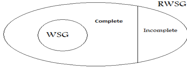
Figure 7.2: Roughly weighted games can be complete or incomplete.
