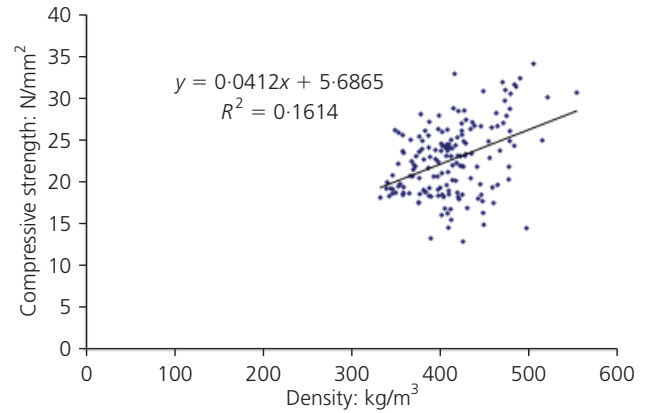
Figure 3. In-grade compressive strength plotted against density
