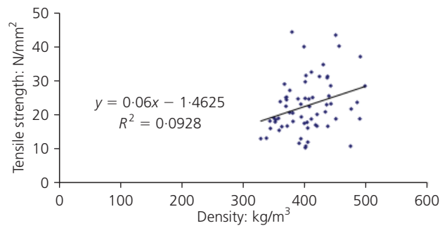
Figure 9. In-grade tensile strength plotted against density
