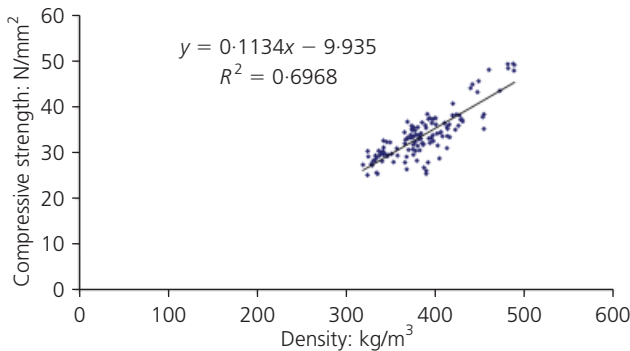
Figure 1. Clear wood compressive strength plotted against density
