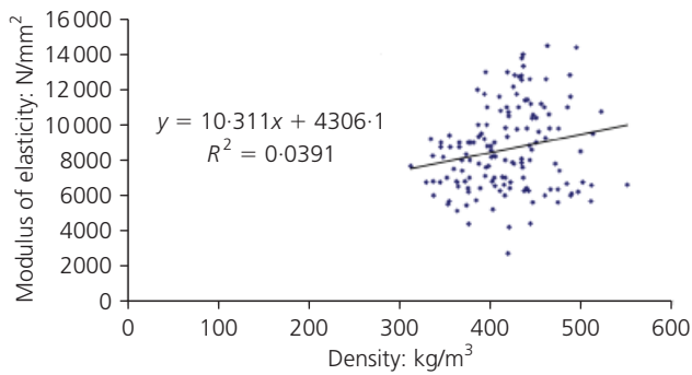
Figure 6. Clear wood modulus of elasticity plotted against density
