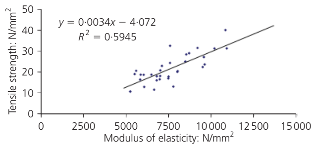
Figure 7. In-grade tensile strength plotted against modulus of elasticity
