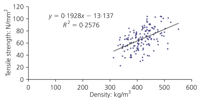
Figure 4. Clear wood tensile strength plotted against density
