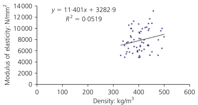
Figure 11. In-grade modulus of elasticity plotted against density
