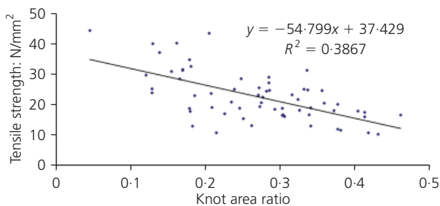
Figure 8. In-grade tensile strength plotted against knot area ratio
