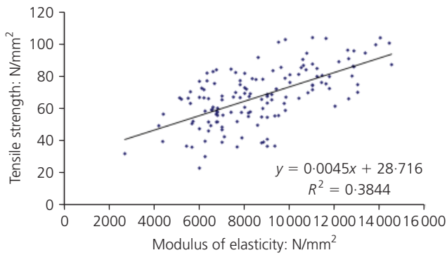
Figure 5. Clear wood tensile strength plotted against modulus of elasticity
