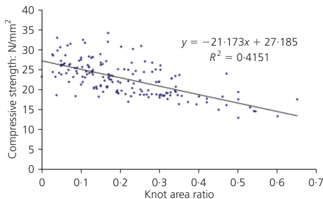
Figure 2. In-grade compressive strength plotted against knot area ratio
