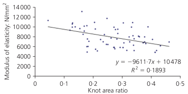
Figure 10. In-grade modulus of elasticity plotted against knot area ratio
