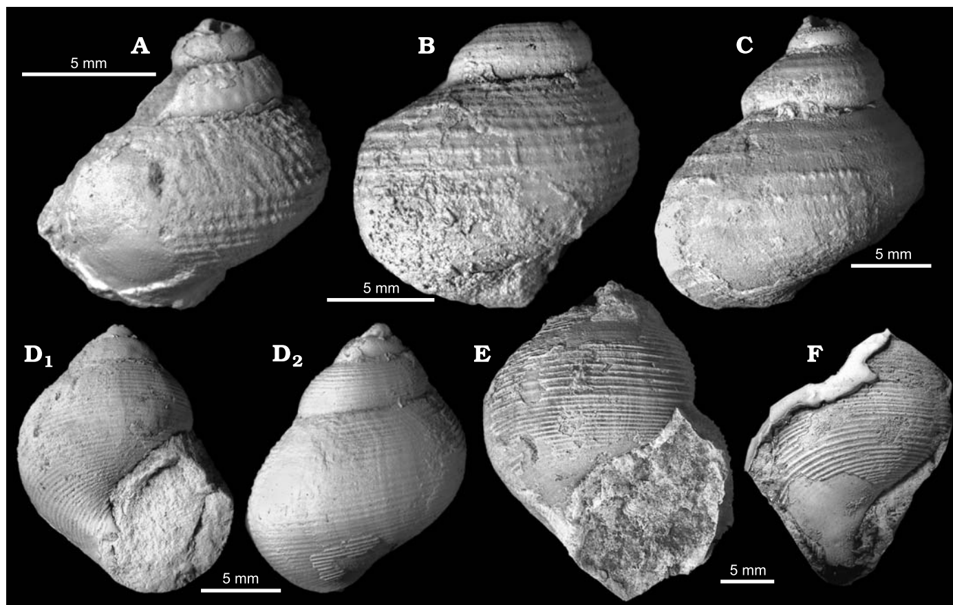
Fig. 7. Abyssochryroid gastropod Paskentana spp. from Late Jurassic and Early Cretaceous seep carbonates in California, USA. A–C. Paskentana berryessaensis sp. nov. A. Holotype (UCMP 555098), small specimen with nodular sculpture from NW Berryessa (Tithonian; site 10). B. Paratype (UCMP 555099), specimen with beaded spiral cords from NW Berryessa (Tithonian; site 10). C. Paratype (UCMP 555100) from Bear Creek (Valanginian; site 4), specimen with spiral sculpture and fine axial growth increments. D–F. Paskentana globosa sp. nov. D. Paratype (UCMP 555101) from Little Indian Valley (Valanginian?; site 6). E. Holotype (CAS 70394), large specimen from Knoxville (Early Cretaceous?, site 9). F. Rubber cast of a last whorl, from Knoxville.
