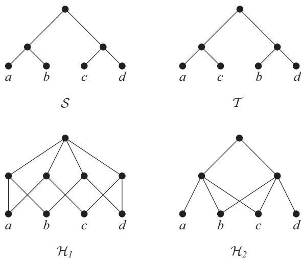
Figure 1. Two rooted binary phylogenetic trees \mathcal{S} and \mathcal{T} and the two hybridization networks \mathcal{H}_1 and \mathcal{H}_2 which explain both trees.
