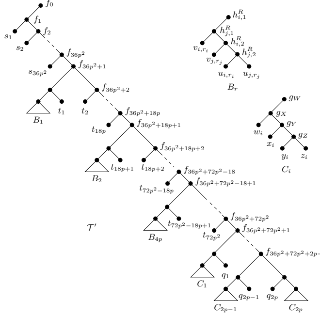
Figure 7: The tree \mathcal{T}' and its subtrees B_r and C_i that are used in the proof of Lemma 4.1.
