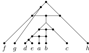
Figure 1: A hybridization network \mathcal{N} with three hybridization vertices and hybridization arcs drawn horizontally.
