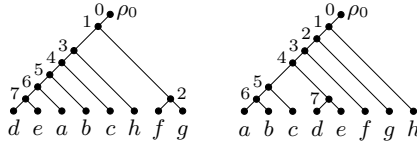
Figure 3: Two planted binary phylogenetic X -trees \mathcal{T} and \mathcal{T}' .
