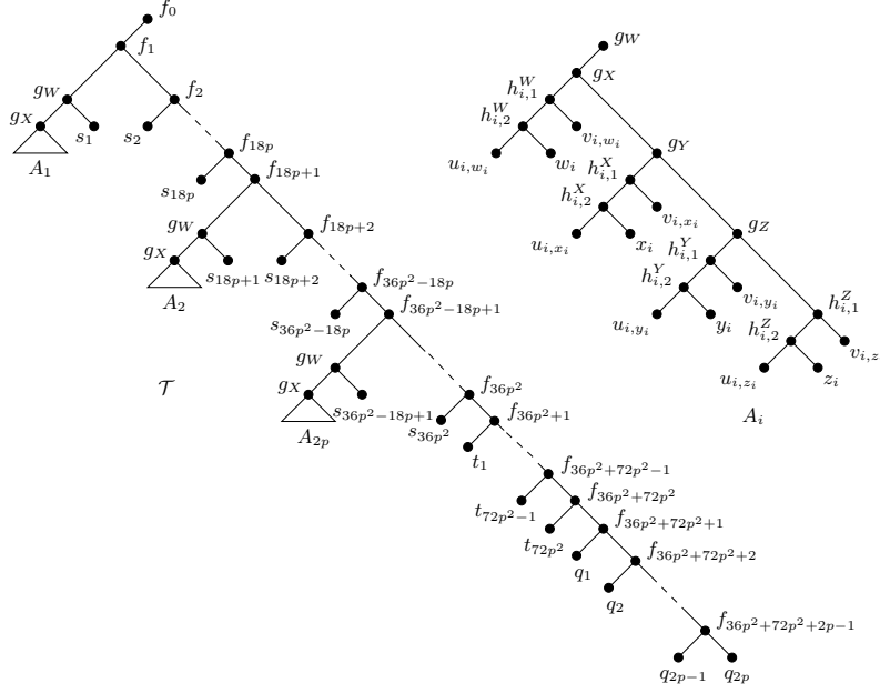
Figure 6: The tree \mathcal{T} and its subtrees A_i that are used in the proof of Lemma 4.1.
