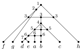
Figure 4: A temporal hybridization network \mathcal{N} . For each internal vertex v a temporal labeling t(v) is given next to v . Note that \mathcal{N} is a minimum temporal hybridization network for the two phylogenetic trees shown in Figure 3.
