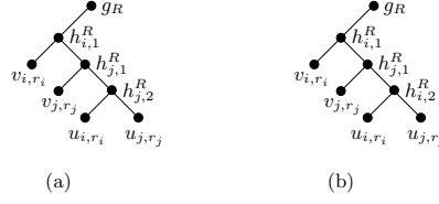
Figure 8: The temporal labeling of the subtree B_r if (a) r_i is contained in a tuple of M and (b) r_j is contained in a tuple of M .
