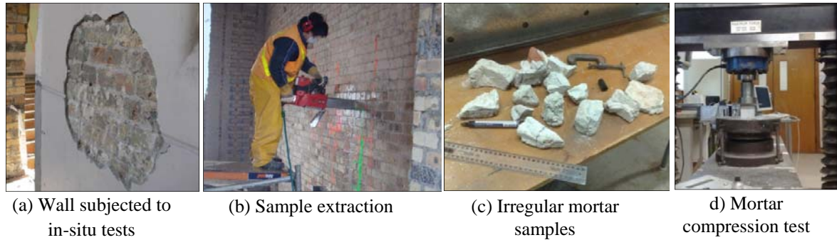
Figure 2: Materials in Wintec Block F building
