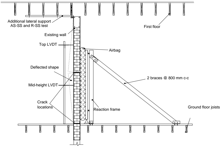
Figure 3: Cross-section of the out-of-plane test setup
