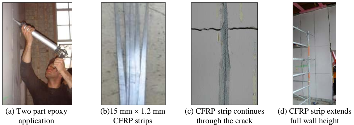
Figure 5: CFRP retrofit application procedure
