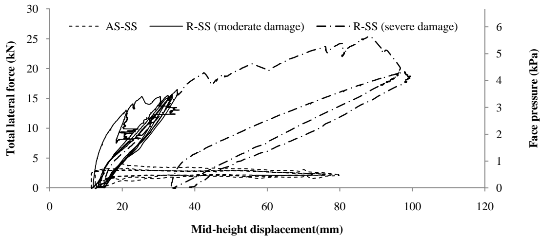
Figure 9: Total lateral force - mid-height displacement response for R-SS test
