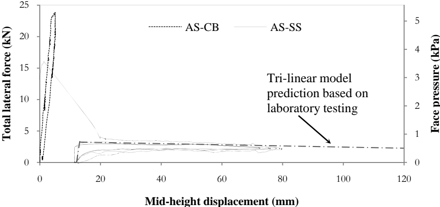
Figure 6: Total lateral force - mid-height displacement response for AS-CB and AS-SS tests
