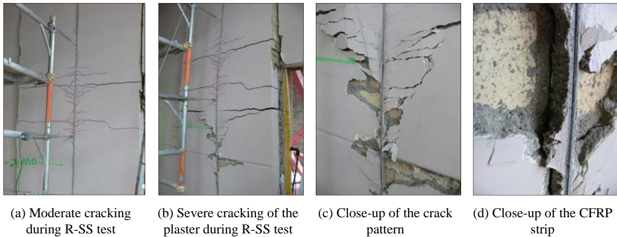
Figure 8: Crack pattern for R-SS test
