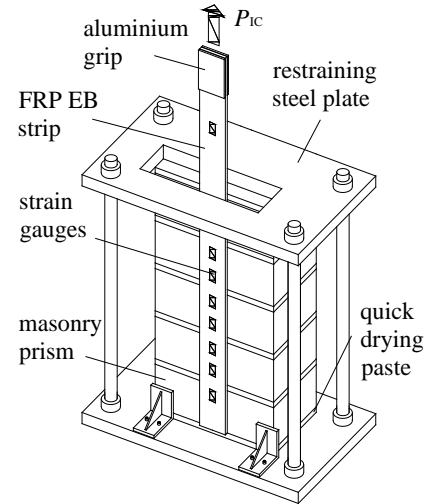
(b) Pull test set-up
