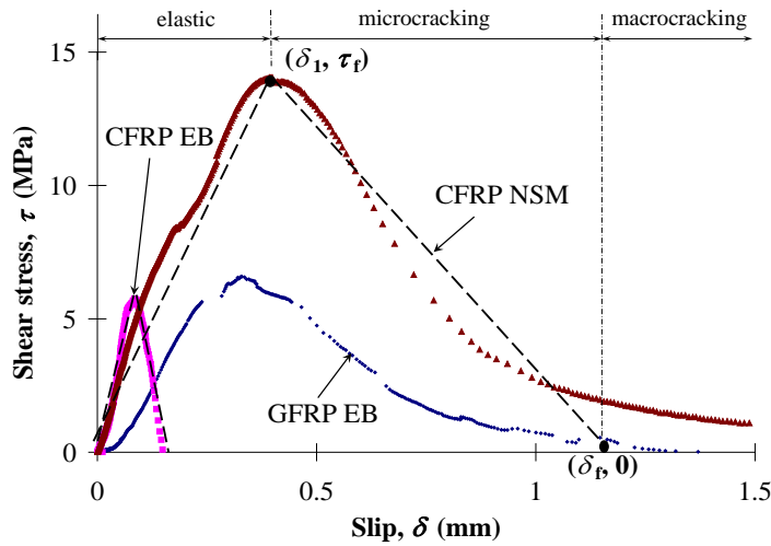
(a) Bond-slip relationship
