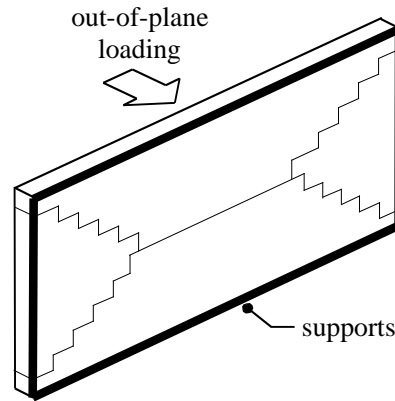
Figure 1. Wall supported along all four edges (Griffith et al. 2005)
