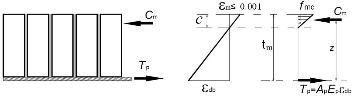
(a) FRP retrofitted masonry section
