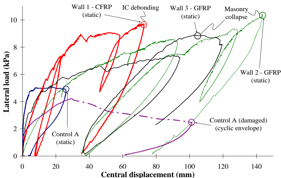
Figure 4. Load-displacement comparison (Willis et al. 2009)
