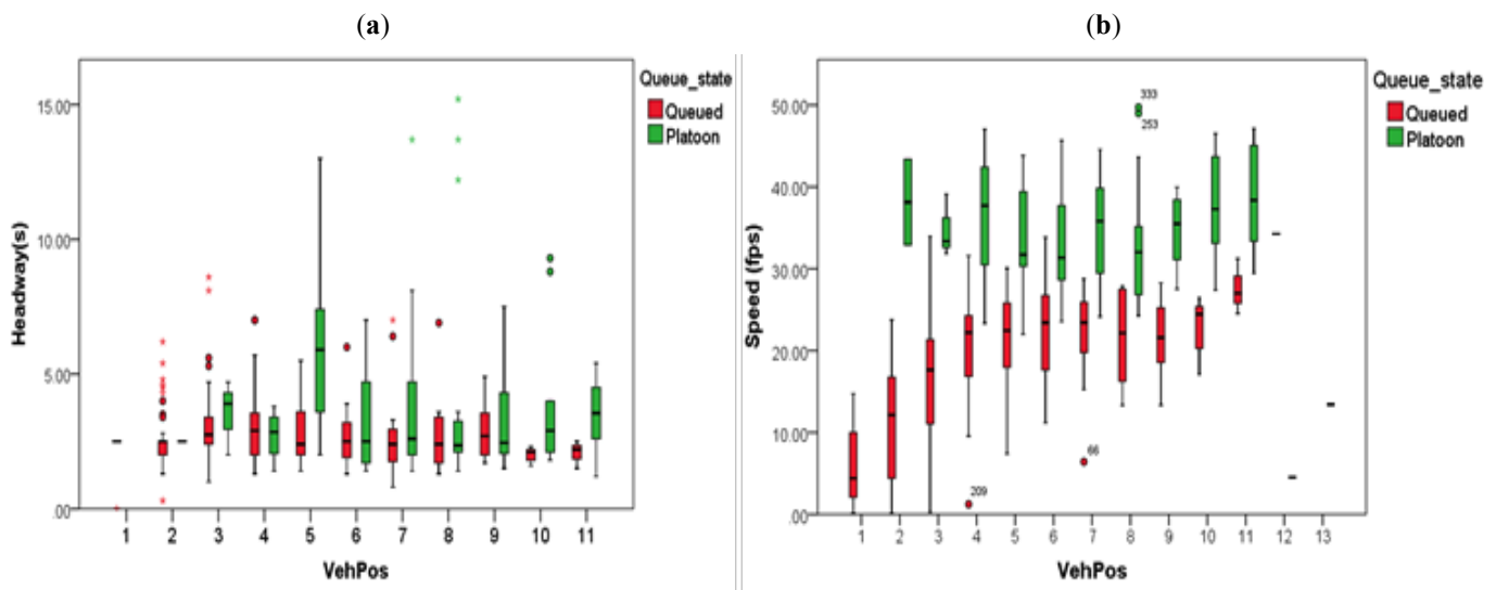
Fig. (4). Variation by vehicle position (a) follow-up headway (b) of vehicle speed.
