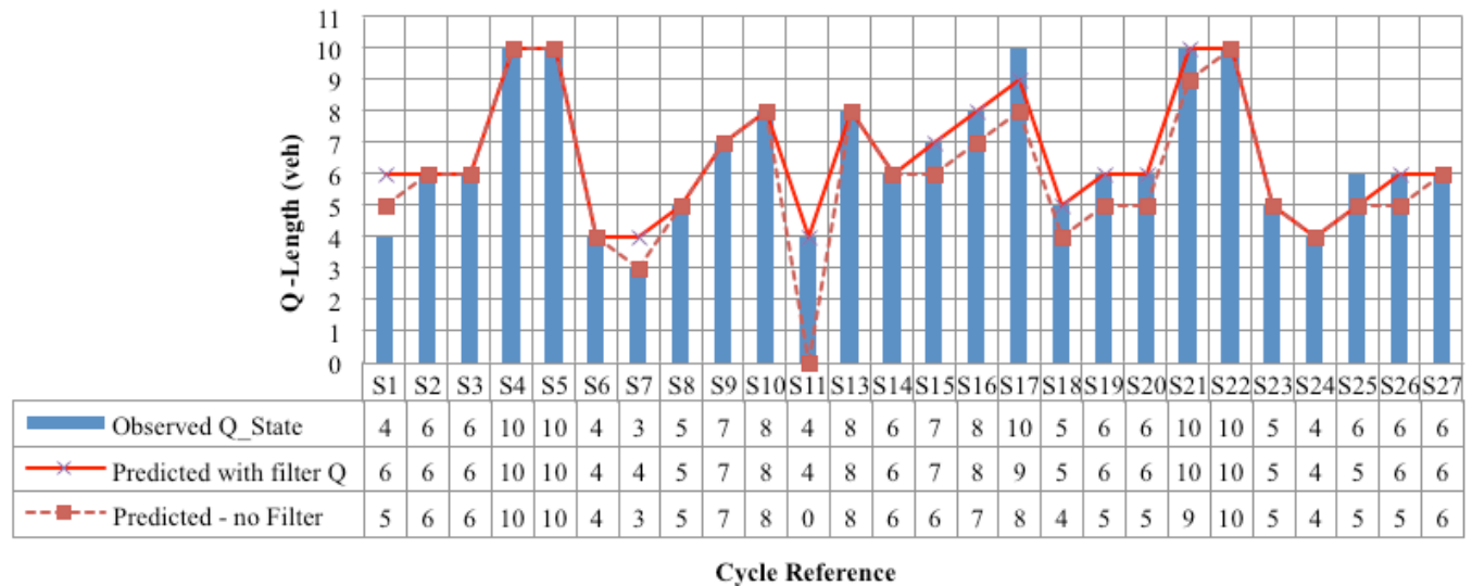
Fig. (6). Model 4 accuracy of SB Q-prediction.
