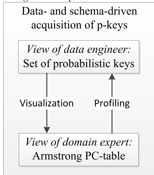
Figure 2: Acquisition framework
