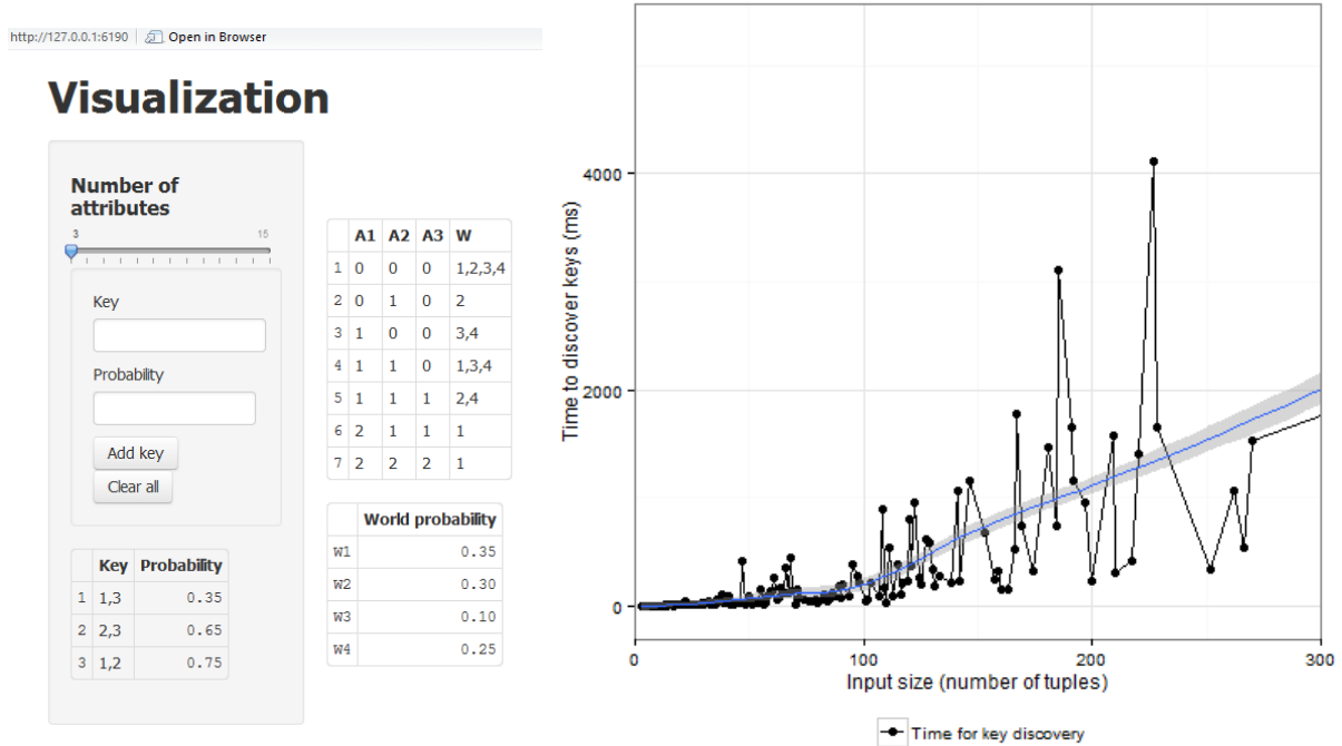
Figure 6: GUI for visualization and times for profiling p-keys
