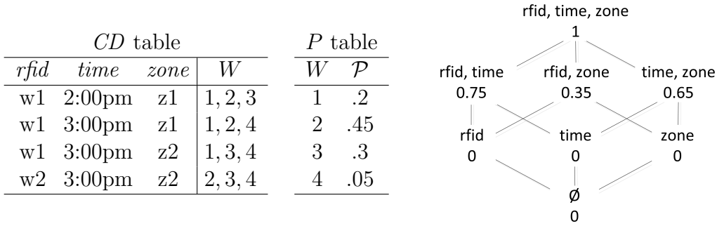
Figure 1: Armstrong PC-table for \{k1_{\geq 0.65}, k2_{\geq 0.75}, k3_{\geq 0.35}\} and its profile of p-keys
