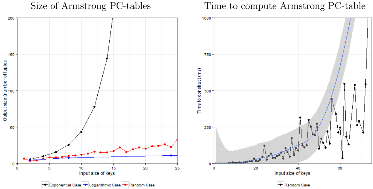
Figure 4: Results of experiments with visualization
