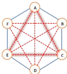
Figure 3: Red triangle in the party graph [3].
