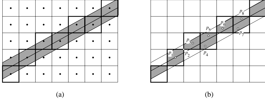
Figure 1: Illustrations to the notions of feasibility. a) Feasible region related to a digital line. b) Feasible parts of pixels forming the feasible set of a digital line.
