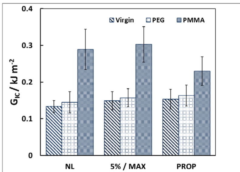
Figure 3. G_{Ic} comparison between virgin and printed composite laminates.
