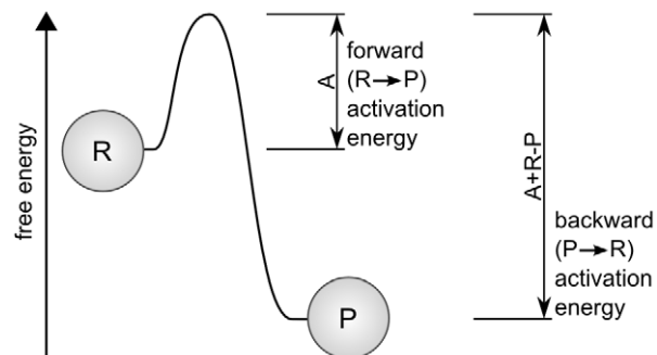
Figure 4. Energy required for a reaction to take place. doi:10.1371/journal.pcbi.1001004.g004
