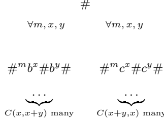
Fig. 6. Automatic presentation of U_{\aleph_0}^2
