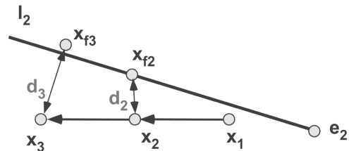
Figure 2: Monocular motion metric. Point e_2 is in the center of the image (an example of a point moving from the focus of expansion). The camera moves forward along its optical axis observing a lateral moving point x_1 \leftrightarrow x_2 \leftrightarrow x_3 . The closest point to x_2 fulfilling the two-view constraints is x_{f2} . The error arising from two-views is the distance d_2 . Transferring the points x_1 and x_{f2} into the third view yields x_{f3} . If the observed 3D point was actually static, x_3 would coincide with x_{f3} . However, the 3D point is moving which causes the trifocal error d_3 . Note: in general, x_1 and x_{f3} do not lie on the epipolar line l_2 .
