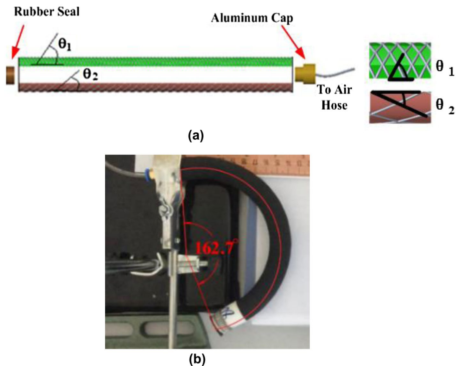
Figure 1. (a) Exploded view of proposed PBA and (b) PBA bending when pressurized.
