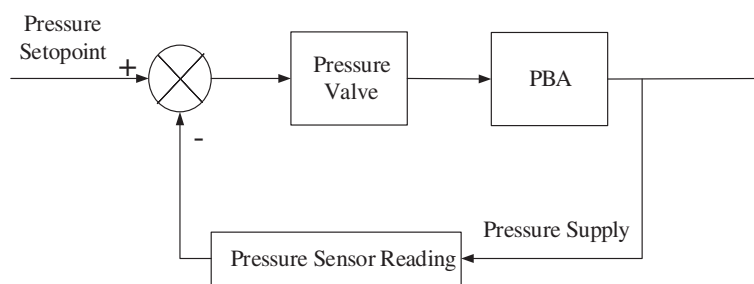
Figure 6. Closed loop control for the input pressure of the soft gripper.
