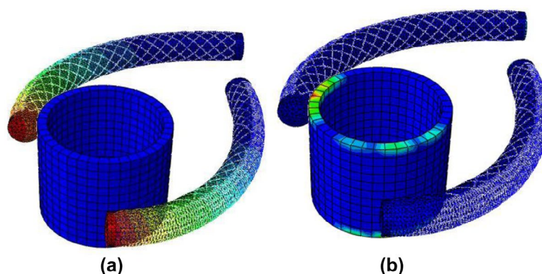
Figure 4. (a) Bending displacement was simulated in Abaqus® 6.14, with red-blue representing high-low displacement respectively and (b) Gripping force was simulated in Abaqus® 6.14, with red-blue representing high-low displacement respectively.
