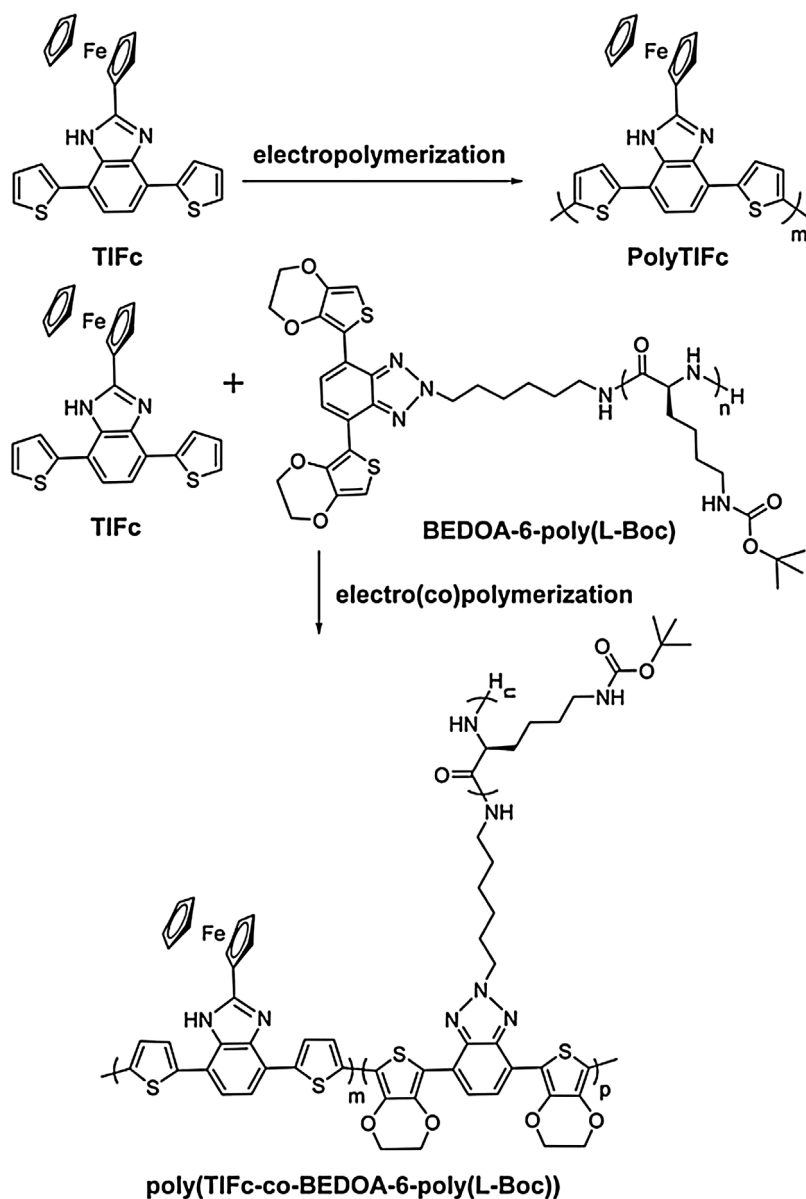
Fig. 10. Synthesis of poly(TIFc) and poly(BEDOA-6-poly(L-Boc)) by electropolymerization. [134], Copyright 2014, Reproduced with permission from the Royal Society of Chemistry.
