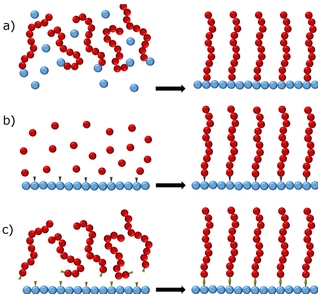
Fig. 3. Generalized categories of graft copolymer synthesis: (a) grafting through (macromonomer approach), (b) grafting from (macroinitiator approach), and (c) grafting to. [38], Copyright 2016. Reproduced with permission from John Wiley & Sons Inc.
