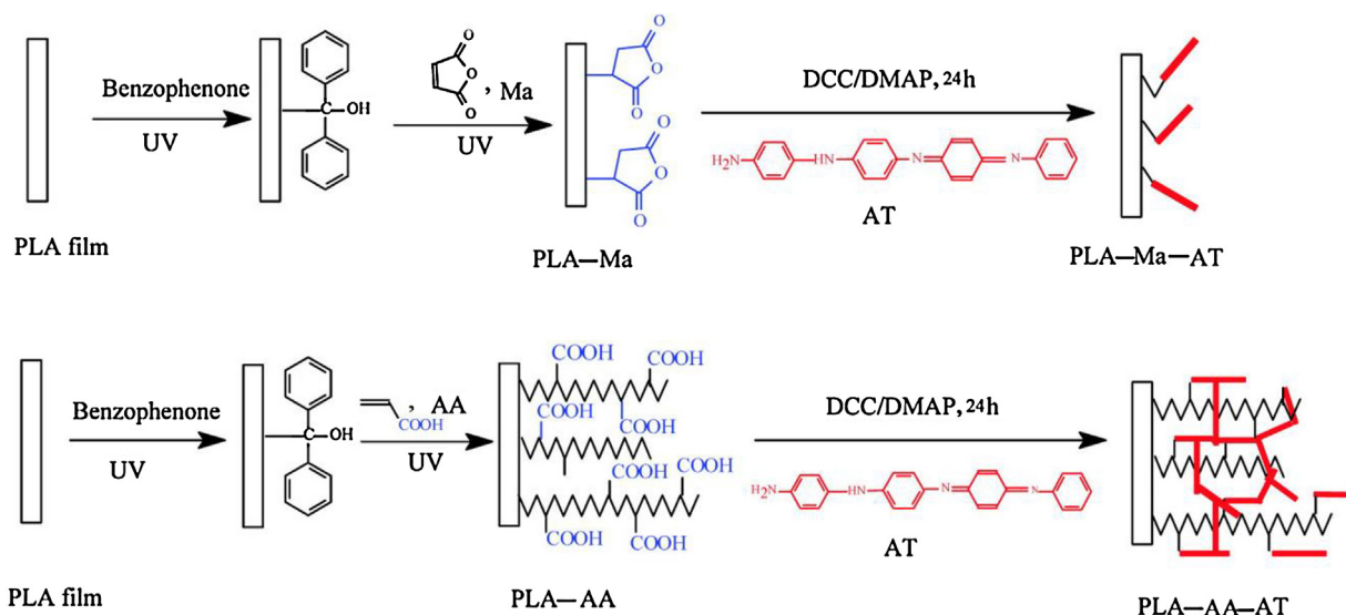
Fig. 8. Surface grafting of poly(lactide) (PLA) films with tetraaniline tetramer (ATA). [127], Copyright 2012, Reproduced with permission from the American Chemical Society.
