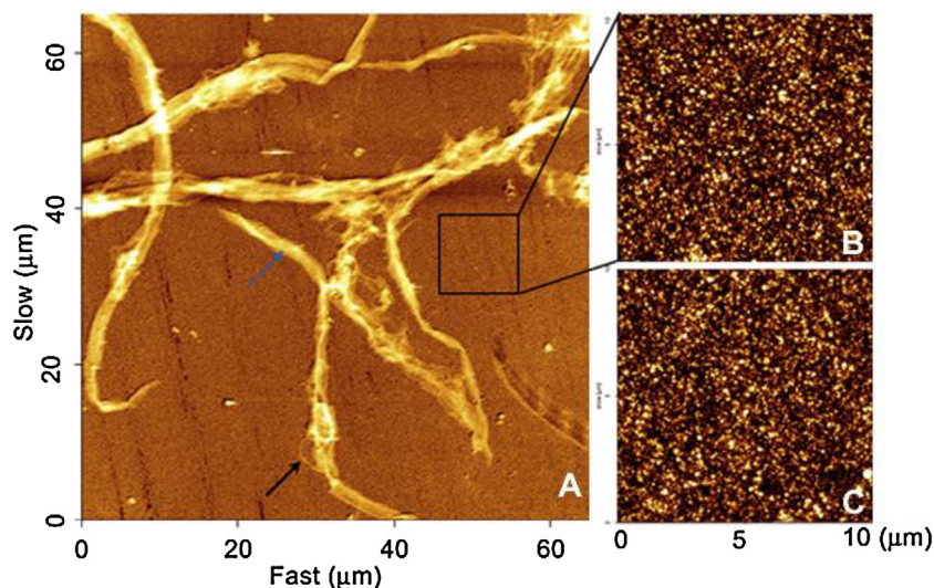
Fig. 2. AFM micrographs of PPy-CS-Col film (A), amplified area on PPy-CS-Col film without collagen fibres (B) and pristine PPy-CS film (C) in PBS. Blue arrow – large fibrous structure, Black arrow – smaller individual fibres. [77], Copyright 2011. Reproduced with permission from Elsevier. (For interpretation of the references to colour in this figure legend, the reader is referred to the web version of this article.)
