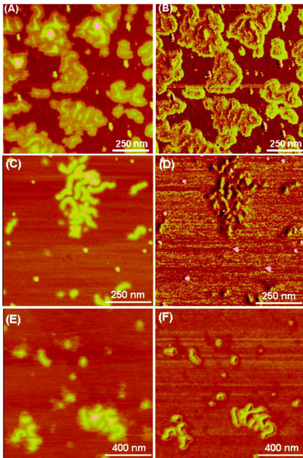
Fig. 4. AFM images (A, C, E: height; B, D, F: phase) of PTh-g-PDMA adsorbed on mica from dilute solution ( 2 \times 10^{-3} \text{ g L}^{-1} ) of toluene (A, B), THF (C, D), and \text{CH}_2\text{Cl}_2 (E, F). Z range (height): 0–10 nm, from dark to bright. [97], Copyright 2008, reprinted with permission from the American Chemical Society.
