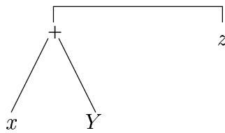
Figure 7: Subtraction operation. Here z and x represent the inputs; Y represents the output. The machine computes z - x . The machine loads into Y a suitable weight, so that the combined weight of x and Y would balance z . Thus, eventually x + Y = z , i.e., Y would represent z - x .
