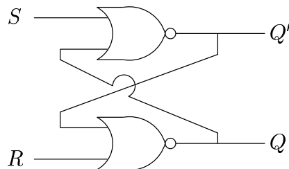
Figure 15: S–R flip-flop constructed using cross coupled NOR gates.
