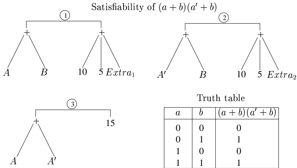
Figure 17: Solving an instance of SAT: The satisfiability of the formula (a + b)(a' + b) is verified. Observe that each of the two clauses have to be true , for the expression to be satisfiable. Machines (1), (2) and (3) work together sharing the variables A , B and A' between them. OR gates (labeled 1 and 2) realize (a + b) and (a' + b) respectively and the NOT gate (labeled 3) ensures that a and a' are “complementary”. Note that the “output” of gates (1) and (2) are set to 10. Now, one has to observe the values eventually assumed by the variable weights A and B (that represent “inputs” of OR gate (1)). Given the assumptions already mentioned, one can easily verify that the machine will balance , assuming one of the two following settings: (i) A = 5 , B = 10 , ( Extra_1 = 0 , Extra_2 = 5 ) or (ii) A = 10 , B = 10 , ( Extra_1 = 5 , Extra_2 = 0 ). These are the only configurations that make the machine balanced. In situations when both the left pans of gate (1) assume 10, Extra_1 will automatically assume 5 to balance off the extra weight on the left side. ( Extra_2 plays a similar role in gate (2).)
