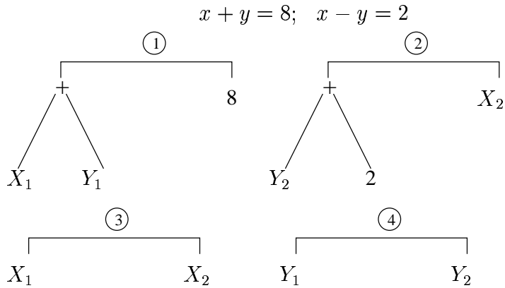
Figure 10: Solving simultaneous linear equations. The constraints X_1 = X_2 and Y_1 = Y_2 will be taken care of by balance machines (3) and (4). Observe the sharing of pans between them. The individual machines work together as a single balance machine.
