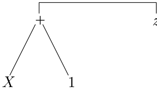
Figure 4: Increment operation. Here x represents the input; Z represents the output. The machine computes increment(x) . Both x and ‘1’ are fixed weights clinging to the left side of the balance machine. The machine eventually loads into Z a suitable weight that would balance the combined weight of x and ‘1’. Thus, eventually Z = x + 1 , i.e., Z represents increment(x) .
