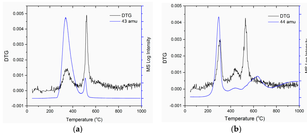
Figure 7. Thermogravimetric analysis combined with mass spectroscopy (TGA-MS). (a) DTG curve of PIM-CONH 2 overlaid with MS trace of m/z 43 amu and (b) DTG curve of C-PIM overlaid with MS trace of m/z 44 amu.
