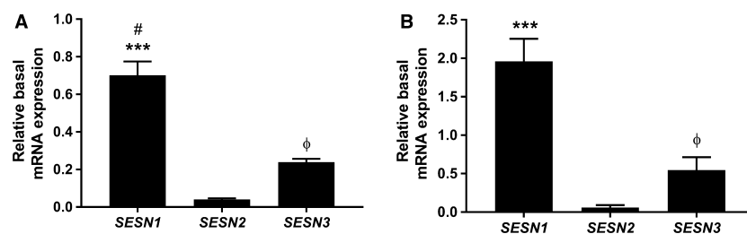
Figure 3. Basal expression of Sestrin paralogs. The basal mRNA expression of SES1 , 2 , 3 in the acute (A) and chronic (B) study. Data are expressed as means \pm SEM. ***Difference between SES1 and SES2 ( P < 0.001 ). #Difference between SES1 and SES3 ( P < 0.05 ). \phi Difference between SES3 and SES2 ( P < 0.05 ).
