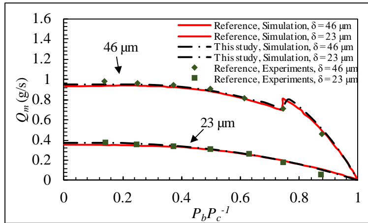
Figure 5. Validation results for the air leakage with P_c = 0.79 MPa, T_c = 300 K [9].
