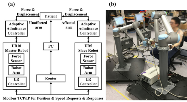
FIGURE 2. The proposed bilateral system. (a) Block diagram of the bilateral system. (b) A healthy subject with the bilateral system.
