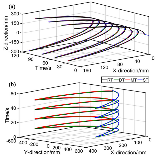
FIGURE 7. Results of the bilateral-passive training protocol. (a) Results of the flexion/extension exercise. (b) Results of the adduction/abduction exercise.
