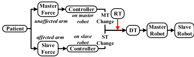
FIGURE 5. Block diagram of the bilateral training protocols.
