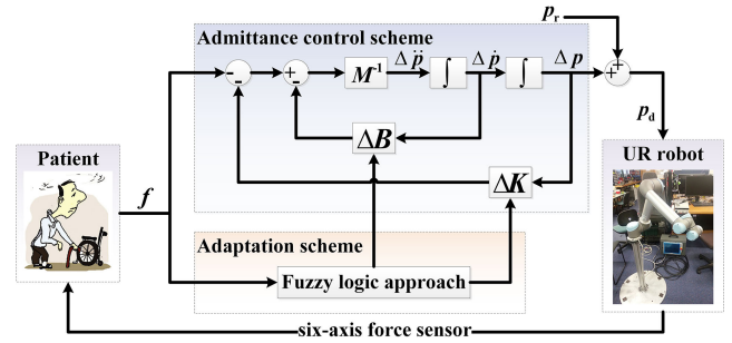
FIGURE 3. Adaptive admittance controller implemented on the UR robot with a patient. f is the interaction force; M is the mass inertia matrix; \Delta B is the change of the damping matrix; \Delta K is the change of the stiffness matrix; \Delta p is the trajectory change; p_r is the reference trajectory; p_d is the desired trajectory.
