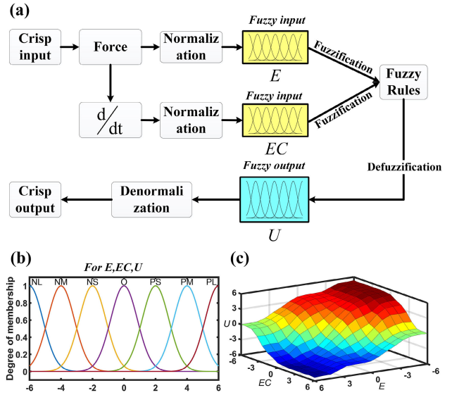
FIGURE 4. The fuzzy logic approach. (a) Block diagram of the fuzzy logic approach. (b) Membership functions for E , EC and U . (c) Surface of fuzzy rules.
