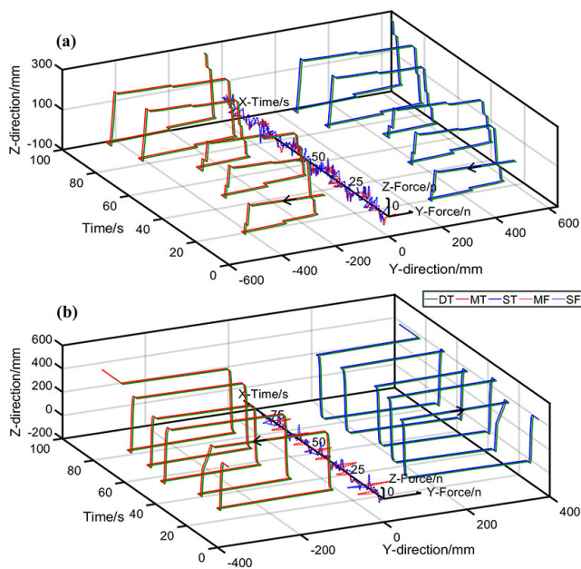
FIGURE 10. Results of the bilateral-self training protocol. (a) Results of the bilateral-self-mimic exercise. (b) Results of the bilateral-self-cooperative exercise.
