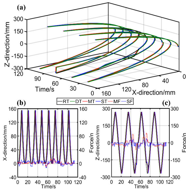
FIGURE 8. Results of the bilateral-active training protocol during the flexion/extension exercise. (a) Results of the flexion/extension exercise. (b) Results of the flexion/extension exercise in the X-direction. (c) Results of the flexion/extension exercise in the Z-direction.
