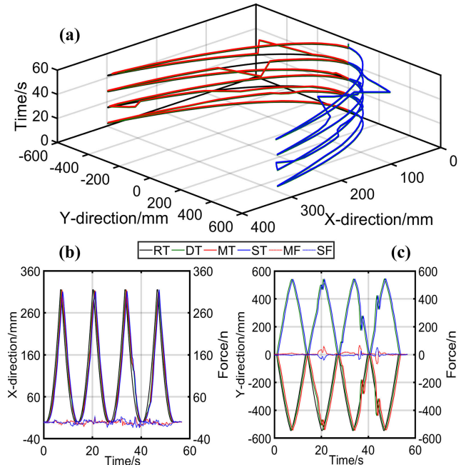
FIGURE 9. Results of the bilateral-active training protocol during the adduction/abduction exercise. (a) Results of the adduction/abduction exercise. (b) Results of the adduction/abduction exercise in the X-direction. (c) Results of the adduction/abduction exercise in the Y-direction.
