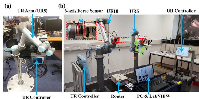
FIGURE 1. The diagrammatic hardware. (a) The UR5. (b) Prototype of the proposed bilateral system.
