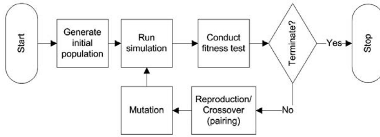
Figure 1 Basic genetic algorithm process
