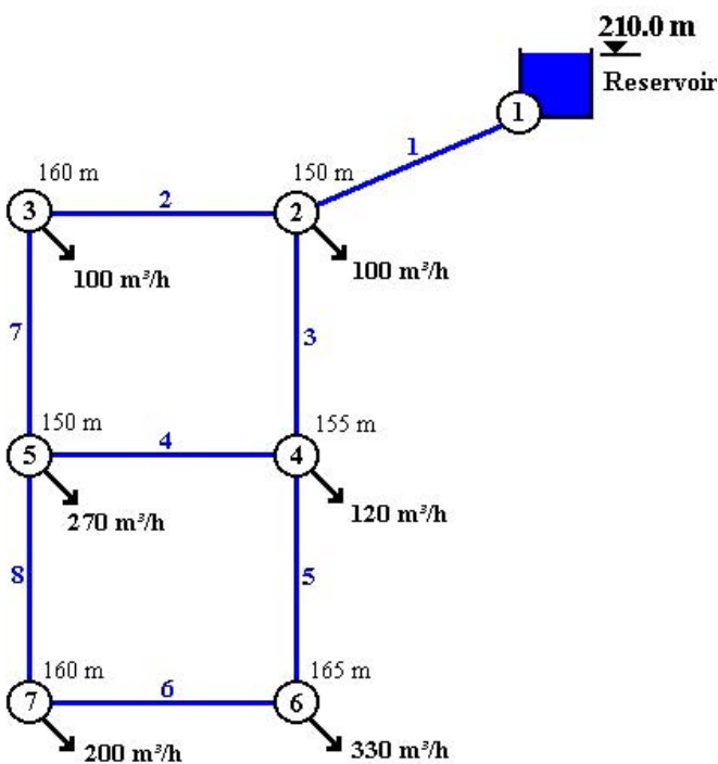
Figure 8 Two-loop network
