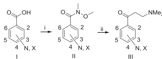
Scheme 2. Synthesis of new pyridyl 3-(dimethylamino)propan-1-one C/D units. Reagents and conditions: (i) \text{COCl}_2 , cat. DMF, DCM, then \text{MeNH}(\text{OMe}) . HCl, pyridine; (ii) vinylMgBr, then \text{Me}_2\text{NH} , THF.
