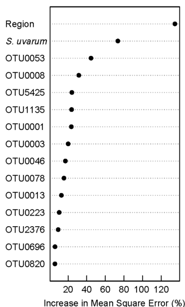
Figure 4. Variable importance as a measure of the percent increase in mean square error when that variable is removed from the random forest analysis for the ratio of 3-mercapto-hexan-1-ol (3MH) and 3-mercapto-hexan-1-ol acetate (3MHA). The taxonomic identification of the OTUs is listed in Table 1. OTUs, operational taxonomic units; S. uvarum , Saccharomyces uvarum .
