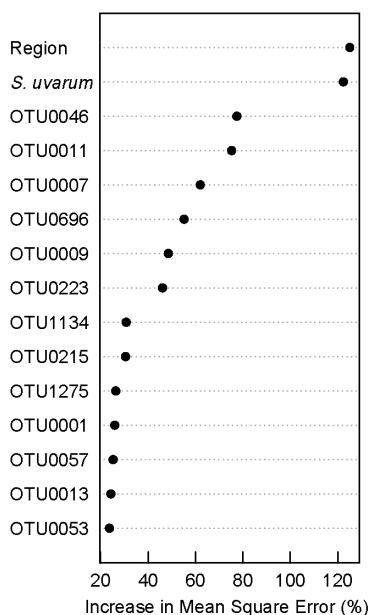
Figure 1. Variable importance as a measure of the percent increase in mean square error when that variable is removed from the random forest analysis for 4-mercapto-4-methylpentan-2-one (4MMP). The taxonomic identification of the OTUs is listed in Table 1. OTUs, operational taxonomic units; S. uvarum , Saccharomyces uvarum .
