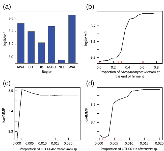
Figure 2. 4-Mercapto-4-methylpentan-2-one (4MMP) partial dependence plots for the top four variables: (a) region; (b) Saccharomyces uvarum at the end of fermentation; (c) proportion of OTU0046 to Penicillium sp. and (d) proportion of OTU0011 to Alternaria sp. identified in the random forest analysis while holding the other variables constant. The tick marks (|) on the x-axis of the panels (b)–(d) represent the deciles of the training data and thus reflect the spread of the data. AWA, Awatere Valley; CO, Central Otago; HB, Hawke's Bay; MART, Martinborough; NEL, Nelson; WAI, Wairau Valley. The location of each of the regions is shown in Figure S1.
