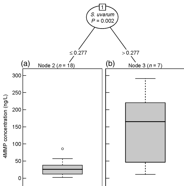
Figure 3. Conditional inference tree explaining the concentration of 4-mercapto-4-methylpentan-2-one (4MMP), performed using the 25 wine samples in Dataset S2. Only three nodes were identified in this analysis, with the proportion of Saccharomyces uvarum at the end of fermentation being identified as the only explanatory variable that significantly affects 4MMP concentration. (a) The 18 wine samples with a proportion of S. uvarum at the end of fermentation less than 0.277 have a significantly lower concentration of 4MMP compared to that of (b) the seven wine samples with a proportion of S. uvarum higher than 0.277 ( P = 0.002 ).
