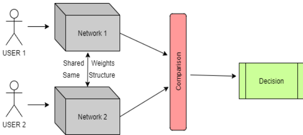
Fig. 1: A typical Siamese neural network structure for biometric system
