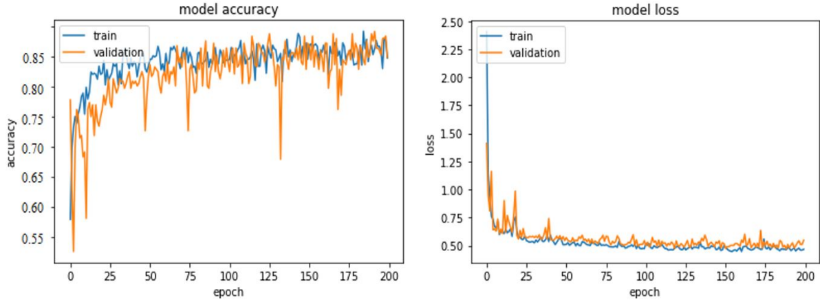
Fig. 3: Accuracy and loss plots: Contrastive loss k=2, n=5
