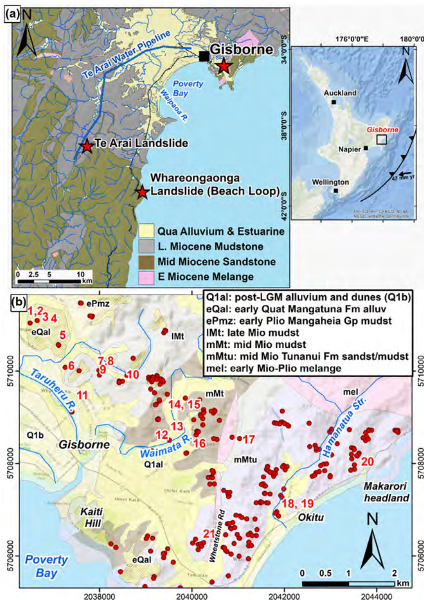
FIGURE 1 (a) Simplified geology of the Gisborne region with Te Arai and Whareongaonga landslides also shown; (b) landslides (red circles) following the November 2021 storm in and around Gisborne city and suburbs (numbers are landslides visited and reported in Table 1), and geological abbreviations are from Mazengarb and Speden (2000).
